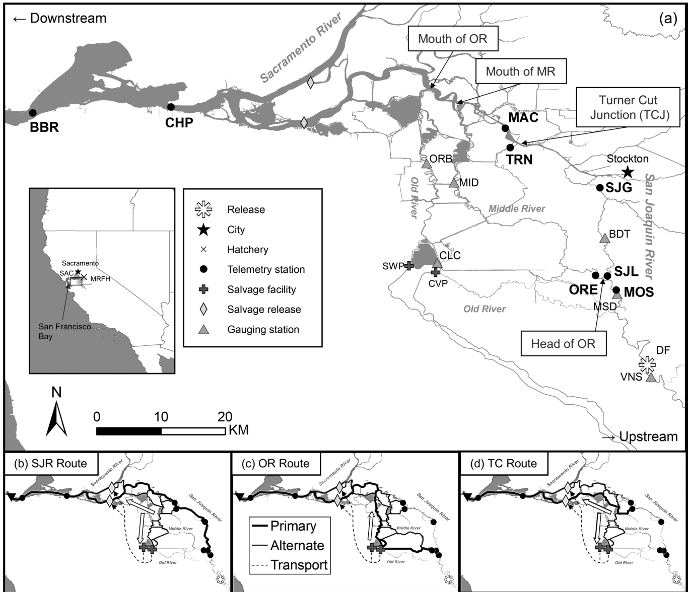
Fig. 1. The study area in the southern Sacramento–San Joaquin River Delta ( a ) and major routes through the study area: San Joaquin River (SJR) route ( b ) and Old River (OR) route ( c ) from the head of OR and Turner Cut (TC) route ( d ) from the Turner Cut Junction (TCJ). Middle River (MR) is a subcomponent of all three routes. White arrows on route maps indicate predominant direction of fish movement in route through the interior Delta. Marked locations are Mokelumne River Fish Hatchery (MRFH; inset map), Durham Ferry (DF) release site, key cities, acoustic telemetry stations, river gauging stations, salvage facilities, and salvage release sites (i.e., after trucking from salvage facilities). Inset map shows state of California, United States (light shading) and the Delta, San Francisco Bay, and Pacific Ocean (dark shading); detailed area is marked with rectangle. Water export and salvage facilities are CVP = Central Valley Project and SWP = State Water Project. Telemetry and gauging stations are defined in Table 2. Map data copyrighted OpenStreetMap contributors (Open Database License), downloaded via Overpass Turbo API ( https://overpass-turbo.eu/ ); Delta boundary data downloaded from https://gis.water.ca.gov/app/boundaries/ . Map created using “rgdal” and “geosphere” packages in R (R Core Team 2020) and ArcMap 10.7.1 (Esri 2011).
