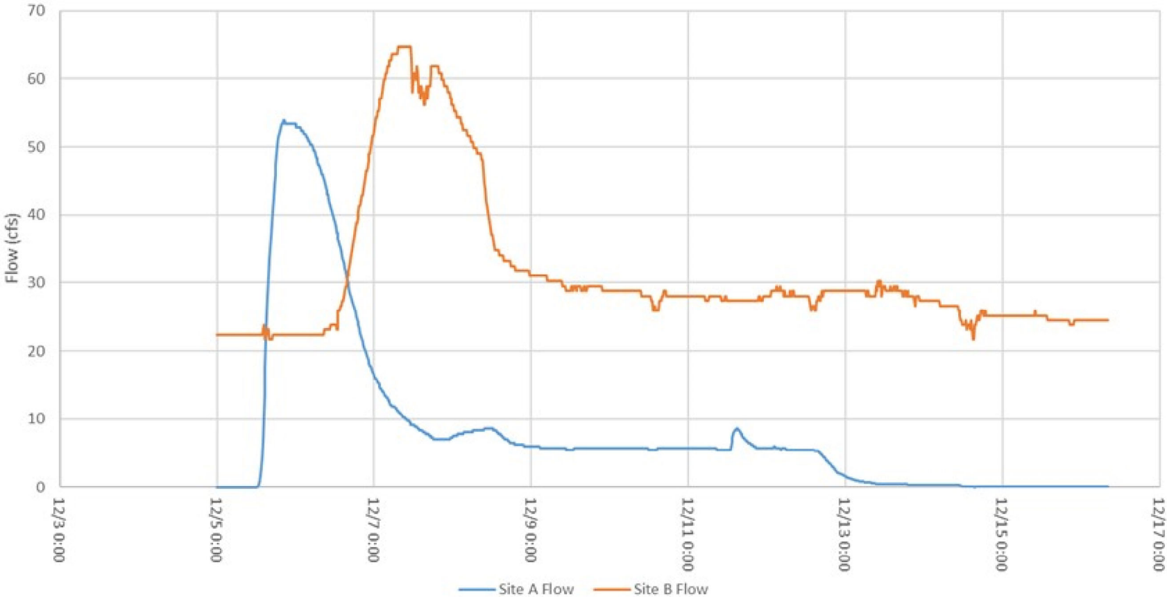
San Luis Drain Flow Measured at Site A and Site B
